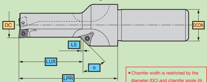
SumiDrill WDX series with Chamfer Edge
