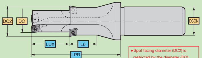
SumiDrill WDX series with Spot Facing Edge
