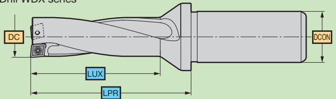
SumiDrill WDX series
